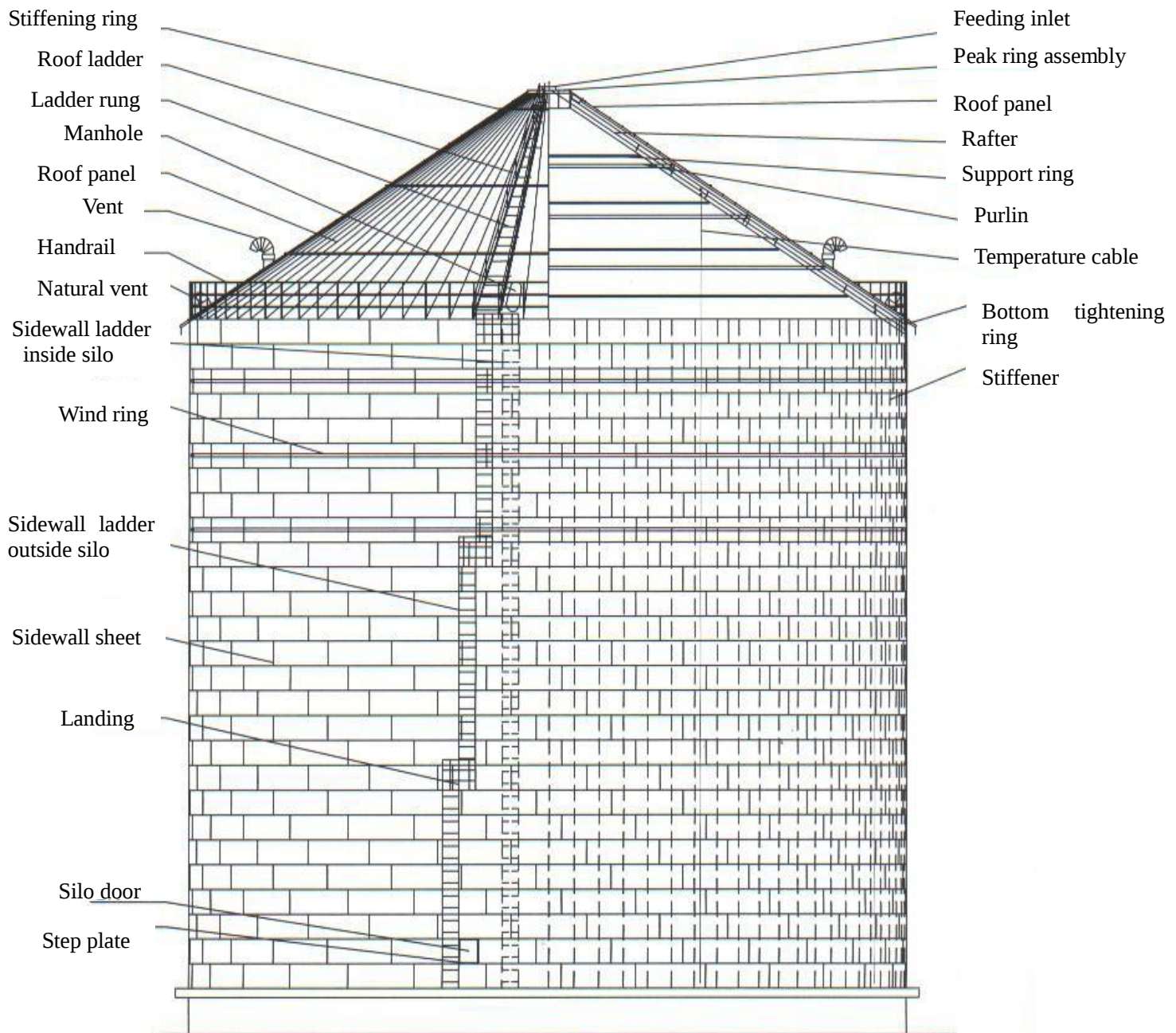
Assembly type steel silo
